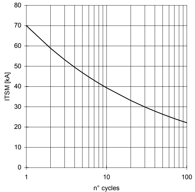
SURGE CHARACTERISTIC T_j = 175\text{ }^\circ\text{C}
